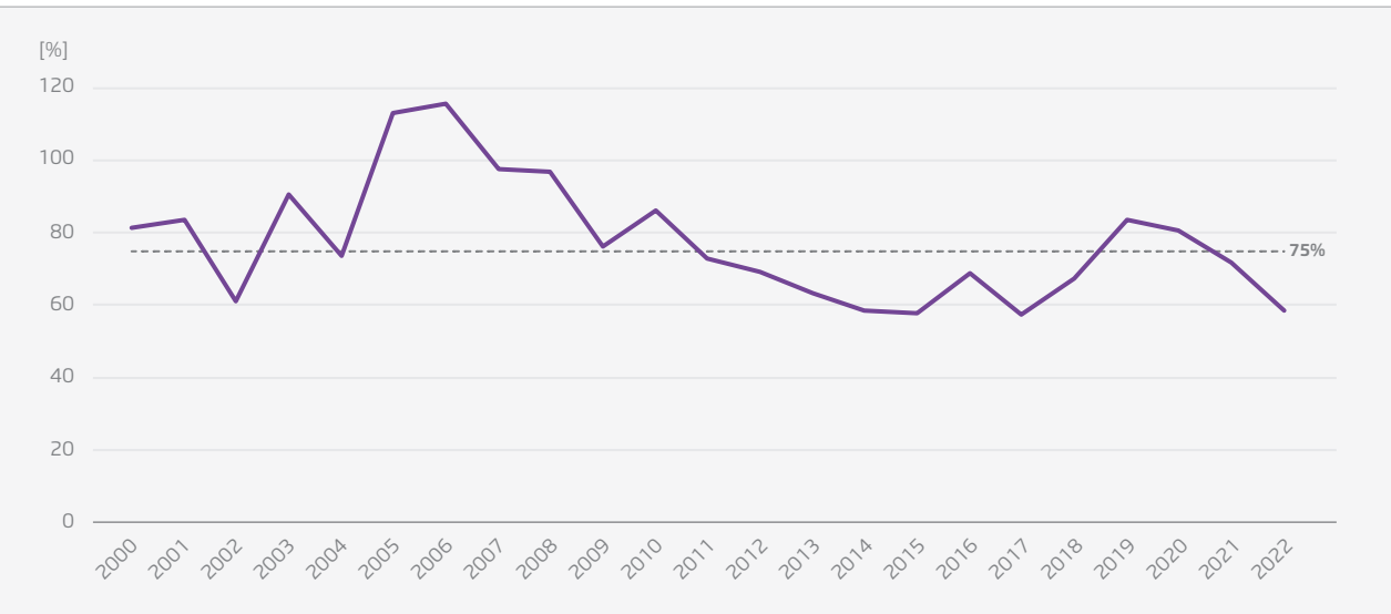
Yearly load factor of coal power generation between 2000–2022 in Vietnam
