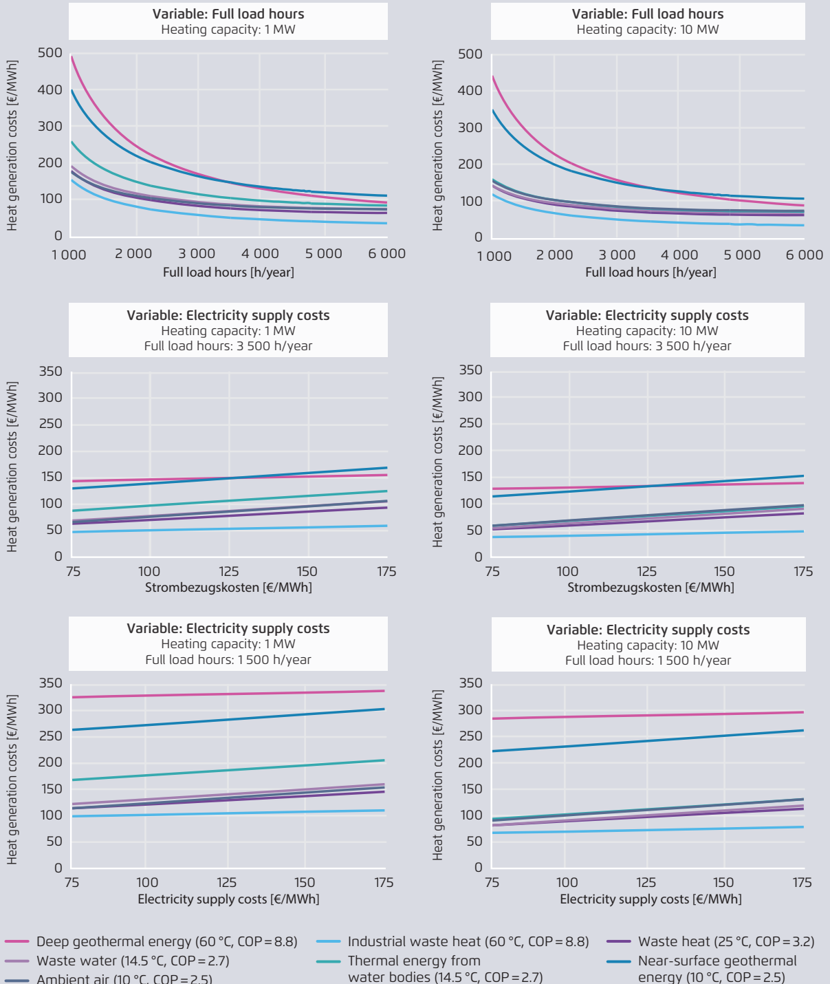
Unit heat production costs in 2030 for different heat sources with varying full load hours and electricity supply costs, for plants with a heating capacity of 1 MW and 10 MW at a sink temperature of 80 °C
